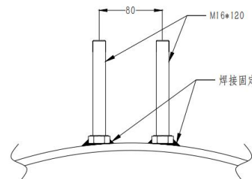
DC110-H/DC210 焊接
