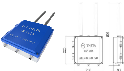
GU100X
