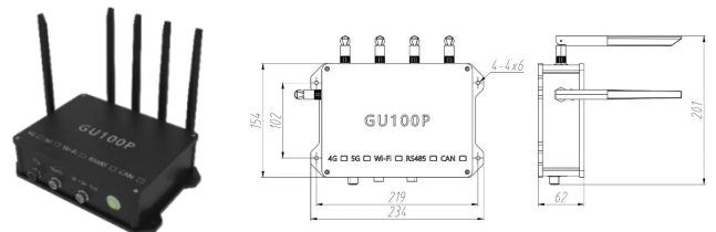
GU100P-5G/-Wi-Fi
